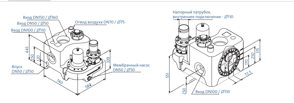
MULTILIFT M
