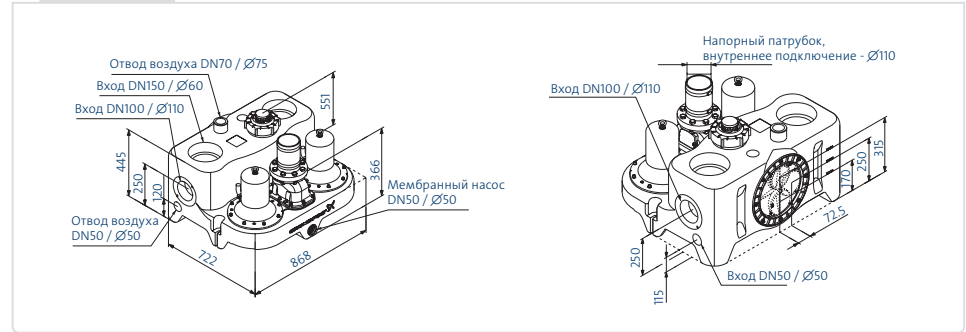
MULTILIFT MD
