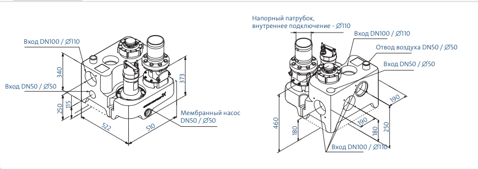
MULTILIFT MSS
