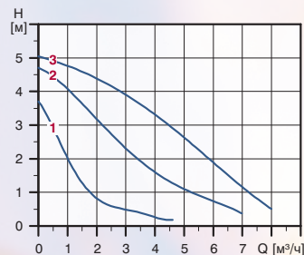
UPS 40-50 F 250
