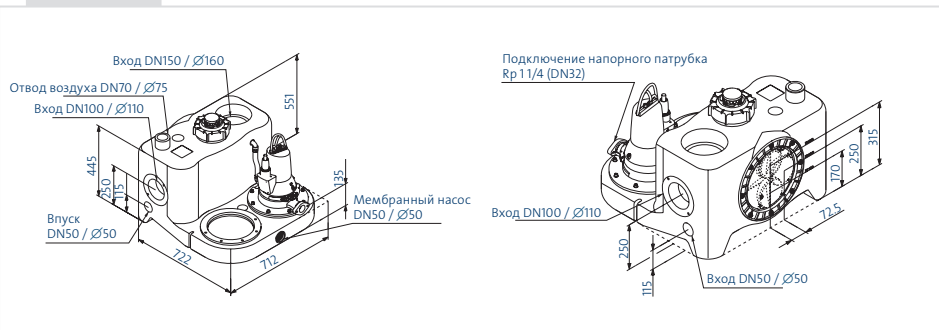
MULTILIFT MOG
