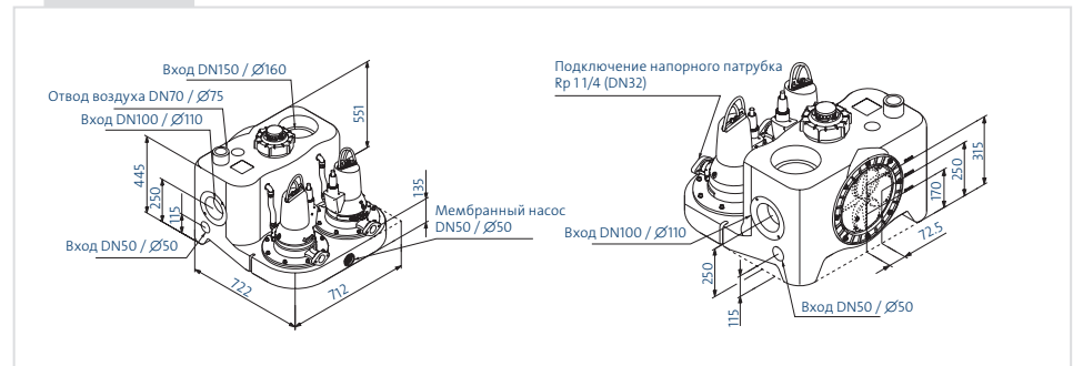
MULTILIFT MDG
